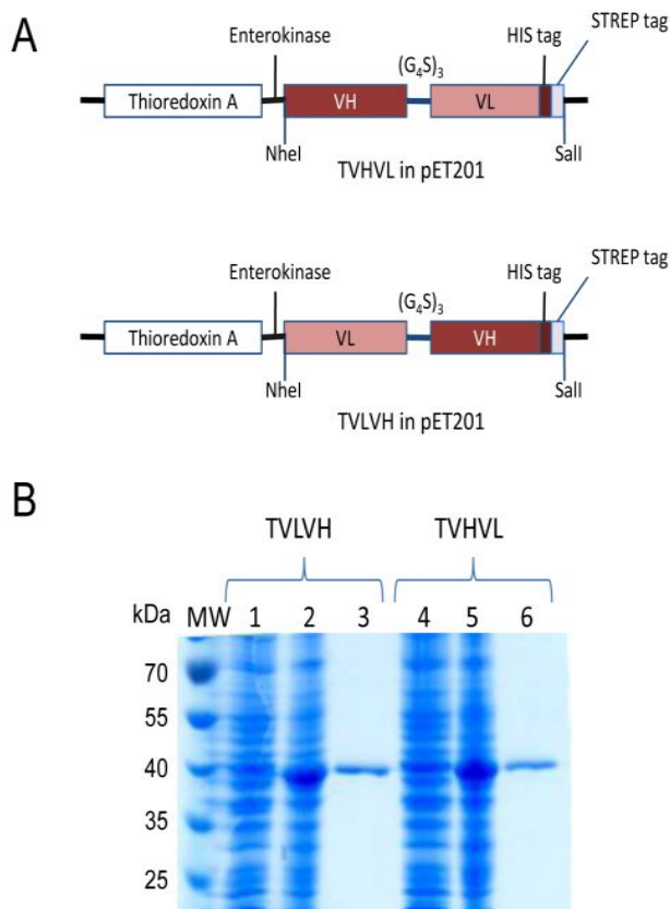
Supplementary file 1: Figure S1. Production of two forms of scFv6-9-1 in fusion with thioredoxin. Schematic diagram of the expression cassettes (A). Expression and purification of TVHVL and TVLVH (B). Total or purified protein extracts from Origami (DE3) strain of Escherichia coli were subjected to 10% SDS-PAGE and stained with Coomassie Brilliant Blue. M, protein molecular weight marker (kDa), line 1 and 4, proteins extracted before IPTG induction; line 2 and 5, proteins extracted after IPTG induction; line 3 and 6, partially purified recombinant TscFv with C-terminal tags. TVHVL and TVLVH have different order of heavy (VH) and light (VL) chains separated by the linker.
